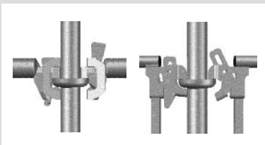
Visible Safety Checks
